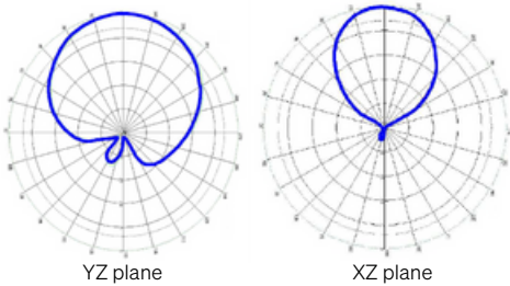
Radiating Pattern
