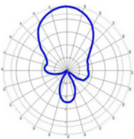
XZ plane
