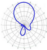
YZ plane
